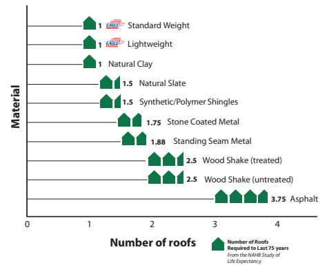
Number of times a re-roof is required over 75 years By choosing Eagle tile you re-roof once avoiding the hassle and expense of multiple re-roofs.
